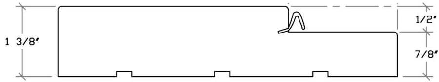
J1 JAMB SINGLE RABBET WITH KERF
