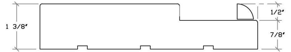
J5 JAMB W. STOP FOR SIDELITE & TRANSOM
