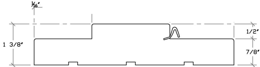
J2 JAMB DOUBLE RABBET WITH KERF * MUST BE 6" OR WIDER
