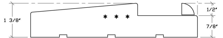
J5 WOODEN SILL SWING IN FOR TRANSOM
