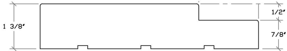
J3 JAMB SINGLE RABBET
