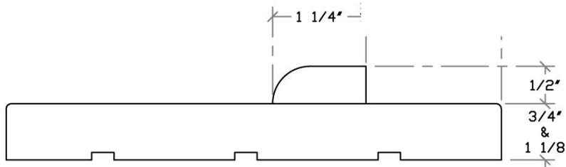
J4 JAMB WITH STOP
