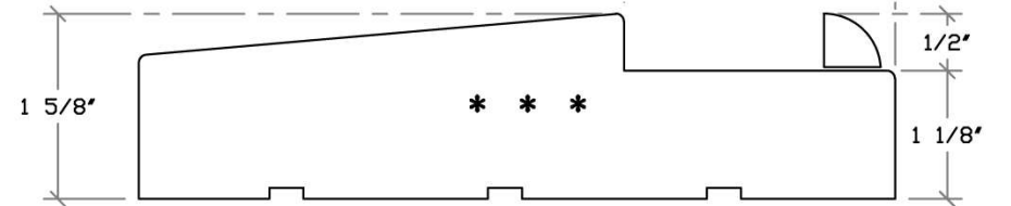
J5 WOODEN SILL SWING IN FOR SIDELITE
