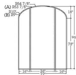
ELLIPTICAL ARCH Single door and two sidelights.
