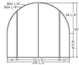
TRUE RADIUS ARCH Double doors and two sidelights.
