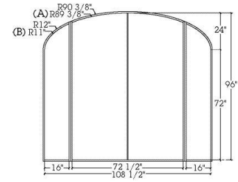
ELLIPTICAL ARCH Double doors and two sidelights.
