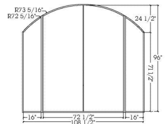
SEGMENT ARCH Double doors and two sidelights.
