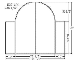
TRUE RADIUS ARCH DOOR AND RECTANGULAR SIDELIGHTS Double doors and two sidelights.
