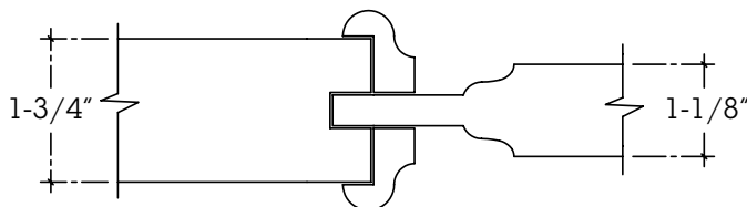
Interior and Exterior Door Profile H3A
