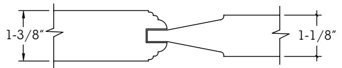
Interior Door Profile H7A
