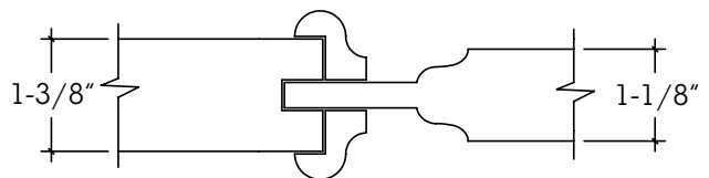
Interior Door Profile H12A
