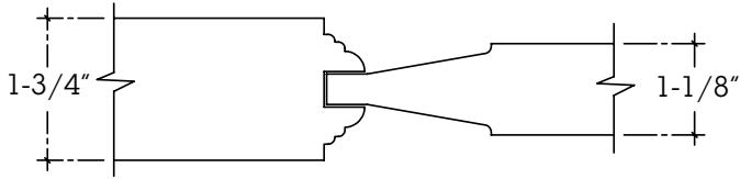
Interior and Exterior Door Profile H1A
