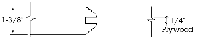
Interior Door Profile H14A
