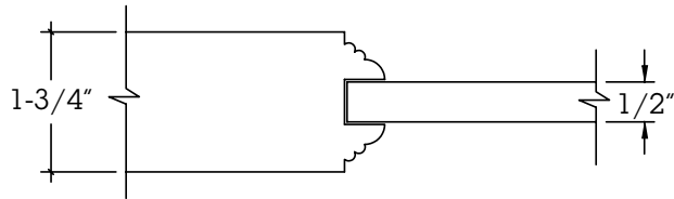
Interior and Exterior Door Profile H2A
