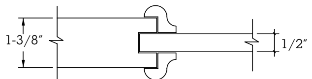
Interior Door Profile H11A
