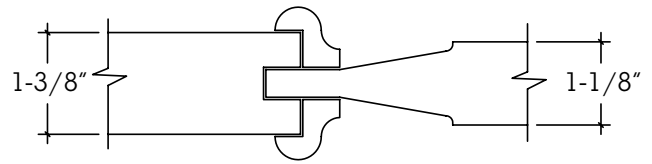
Interior Door Profile H13A
