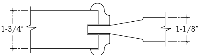
Interior and Exterior Door Profile H6A
