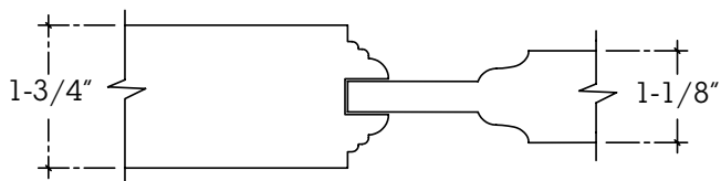
Interior and Exterior Door Profile H5A
