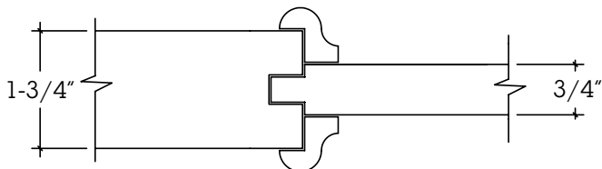
Interior and Exterior Door Profile H4A
