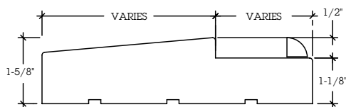
J5 - WOOD SILL FOR SIDELIGHT (with in-swing door)
