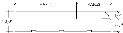
J5 - EXTERIOR SIDELIGHT & TRANSOM (jamb with stop)
