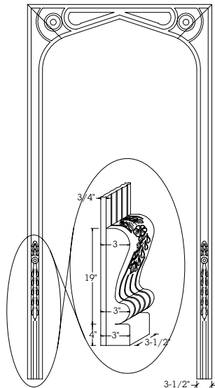
CARVED CASING C7
