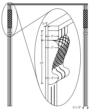
CARVED CASING C11
