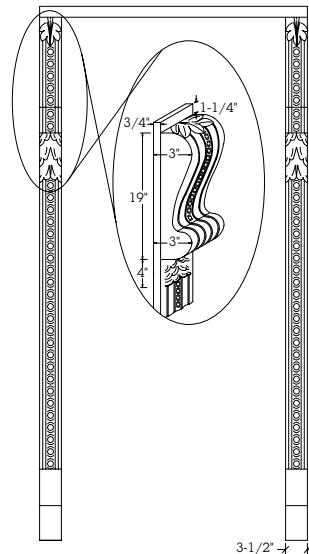
CARVED CASING C8
