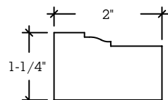
B4 BRICKMOULD
