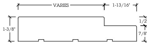
J3 - INTERIOR JAMB (single rabbet)
