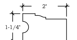
B6 STUCCO BRICKMOULD
