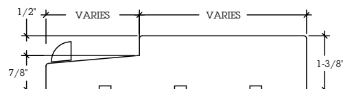
J5 - WOOD SILL FOR SIDELIGHT & TRANSOM (with out-swing door)
